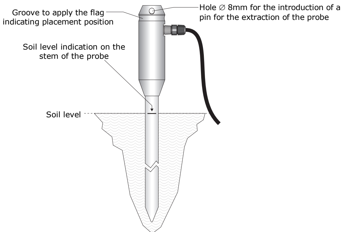
Fig. 2: installation
