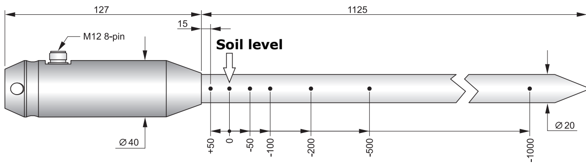
Fig. 1: dimensions of the probe TP32MTT.03 (mm)
