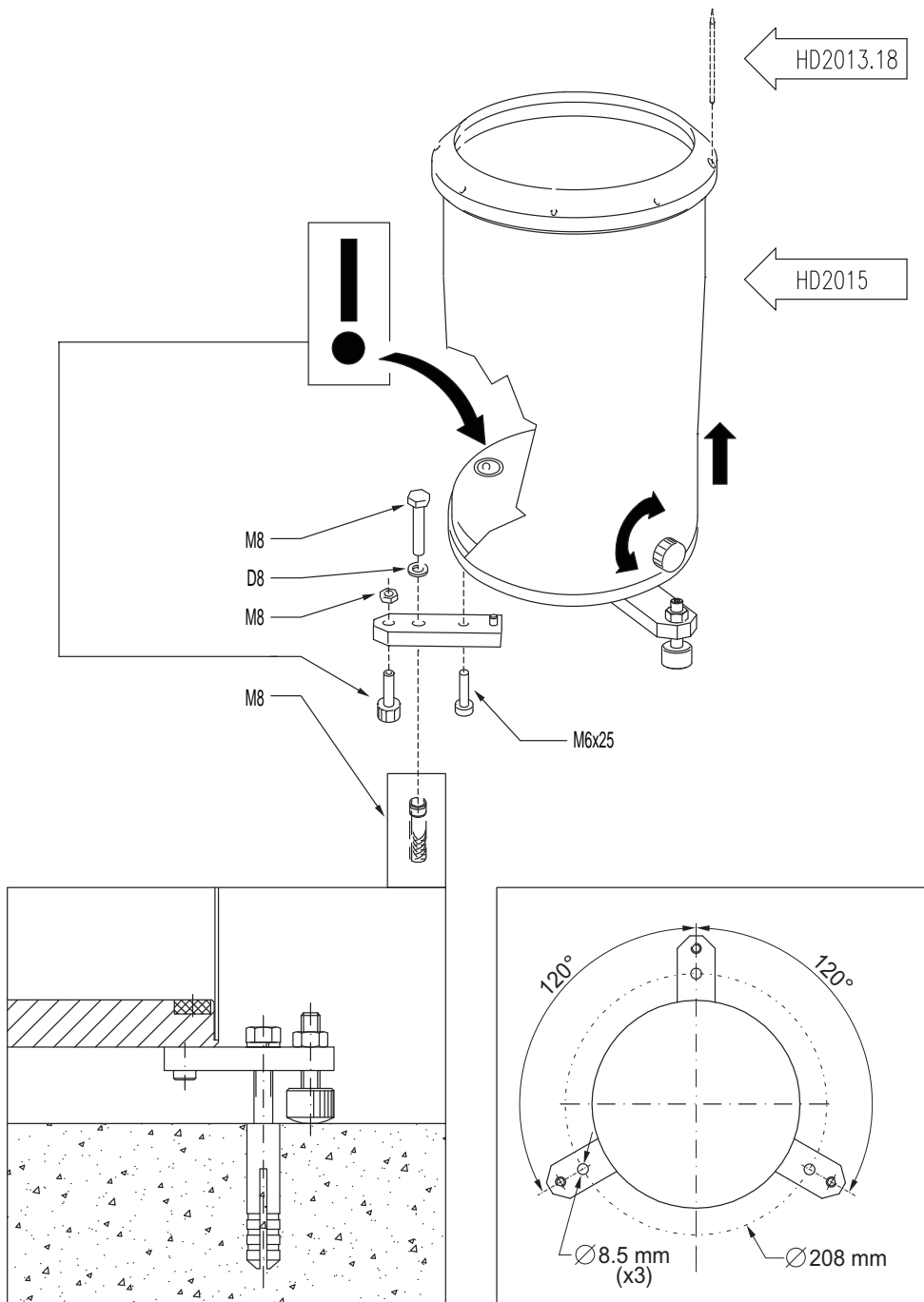
Fig. 7 – Ground installation
