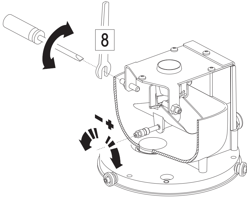
Fig. 5 – Adjustment of the tipping bucket
