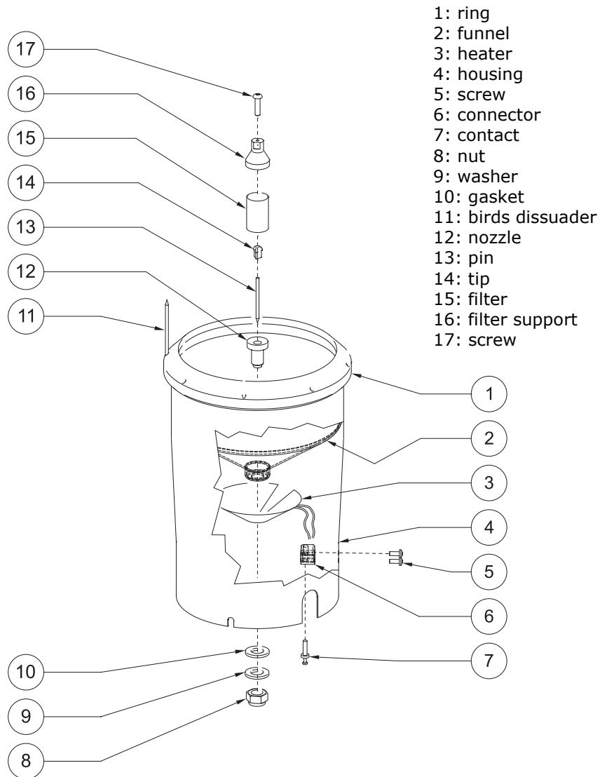
Fig. 9 – Exploded view of the upper part (version with heating)
