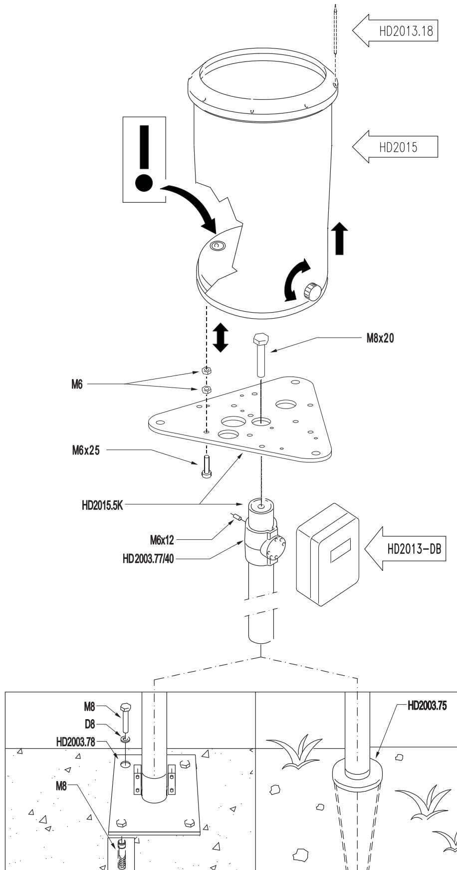
Fig. 8 – Installation raised above ground
