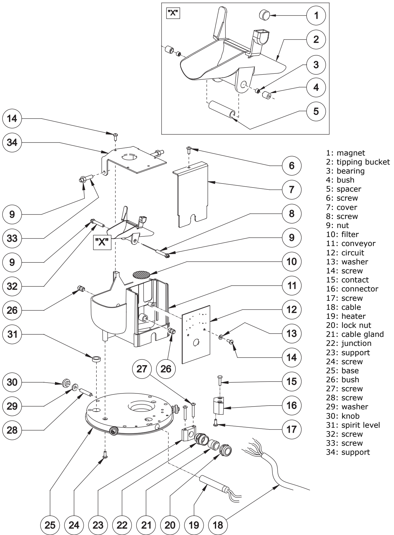
Fig. 10 – Exploded view of the lower part (version with heating)
